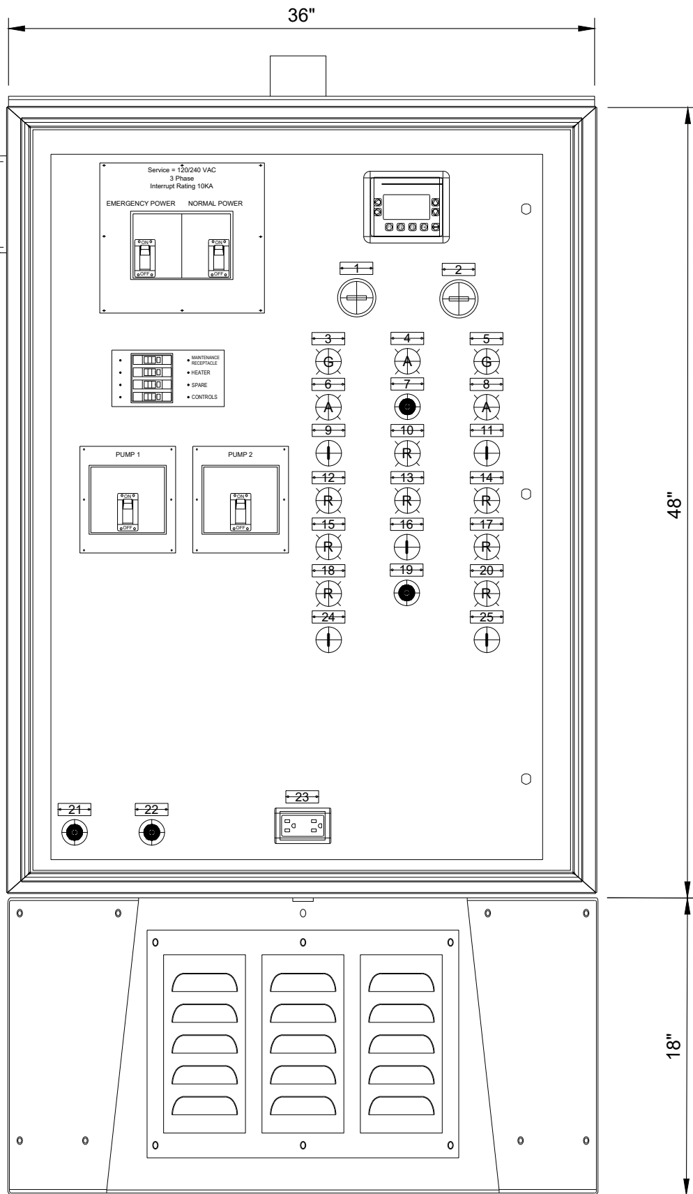
FRONT VIEW WITH OUTER DOOR OPEN
