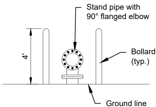
STAND PIPE DETAIL
