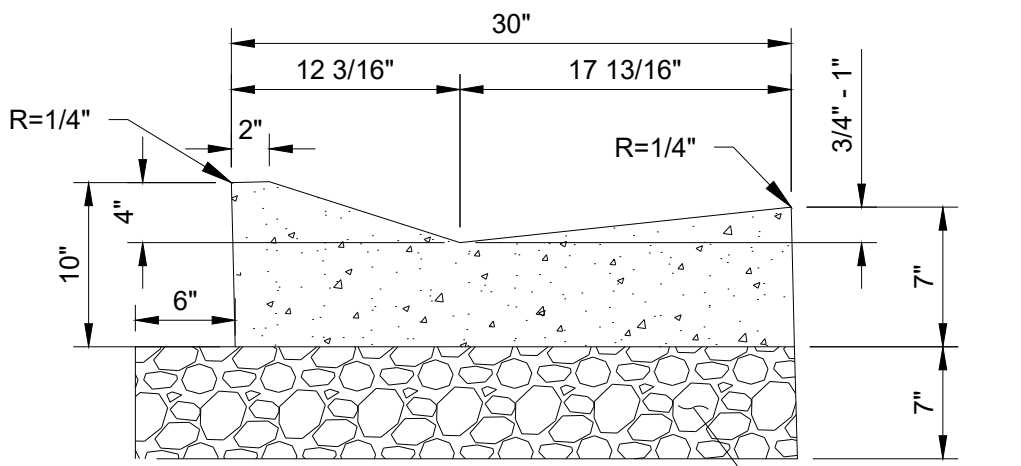
TYPE 2 (MOUNTABLE)
