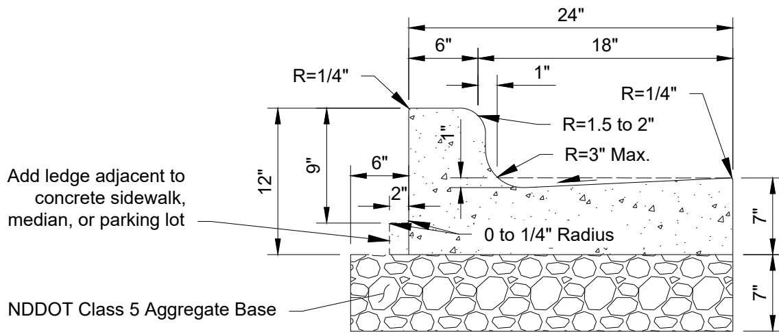
TYPE 1A (INFLOW)
