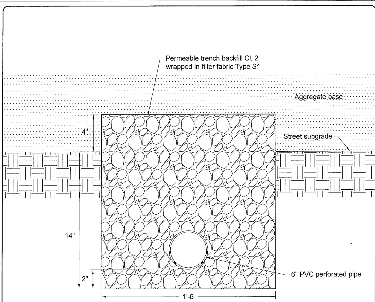
TRENCH DETAIL
