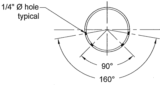
PIPE DETAIL
